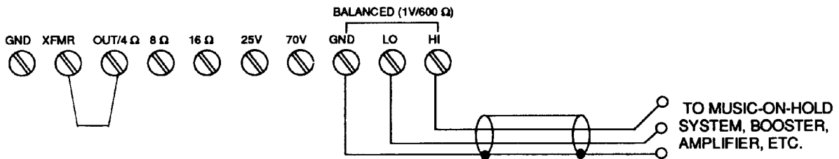
Figure 6. 1 V Balanced Output Connectors
